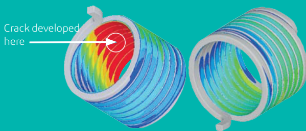
fe-safe fatigue life contour plot
